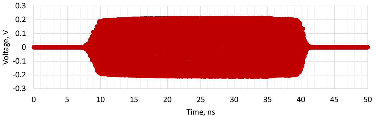
Figure 15: 10 GHz pulse-modulated signal
