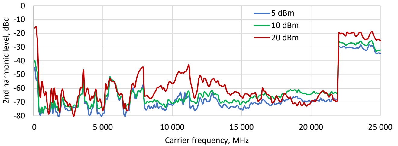
Figure 5: 2nd harmonic levels at different output power levels (20 dBm or maximum power whichever is lower)
