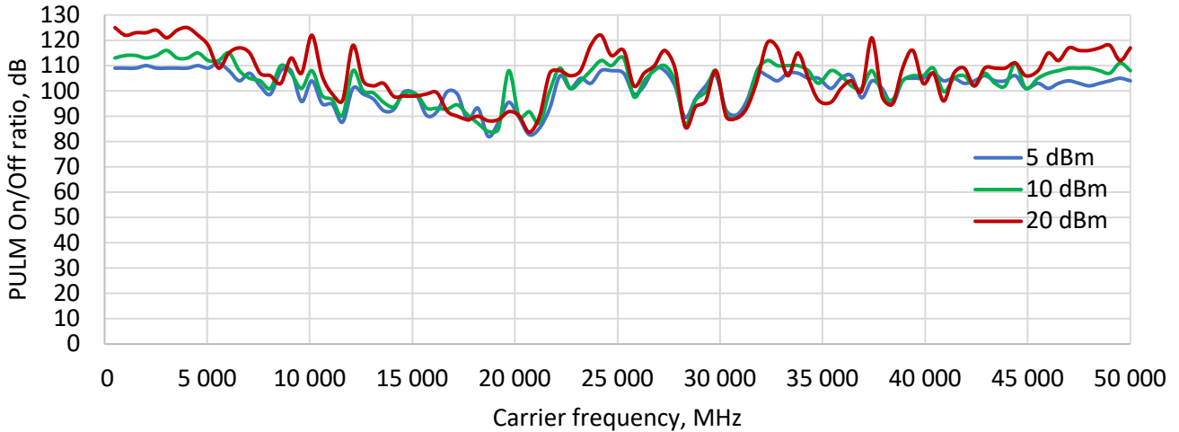
Figure 14: PULM On/Off ratio over frequency at different output power levels (20 dBm or maximum power whichever is lower)
