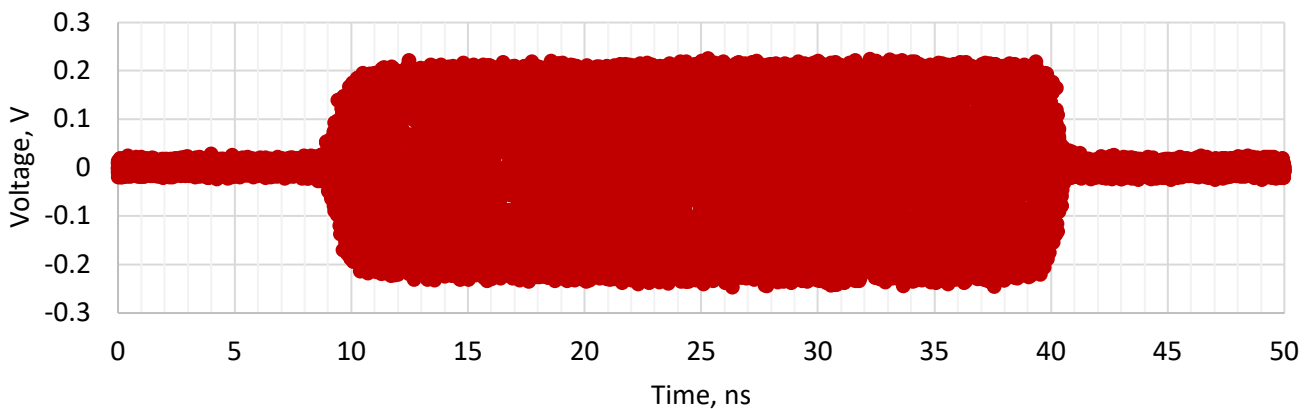
Figure 16: 50 GHz pulse-modulated signal
