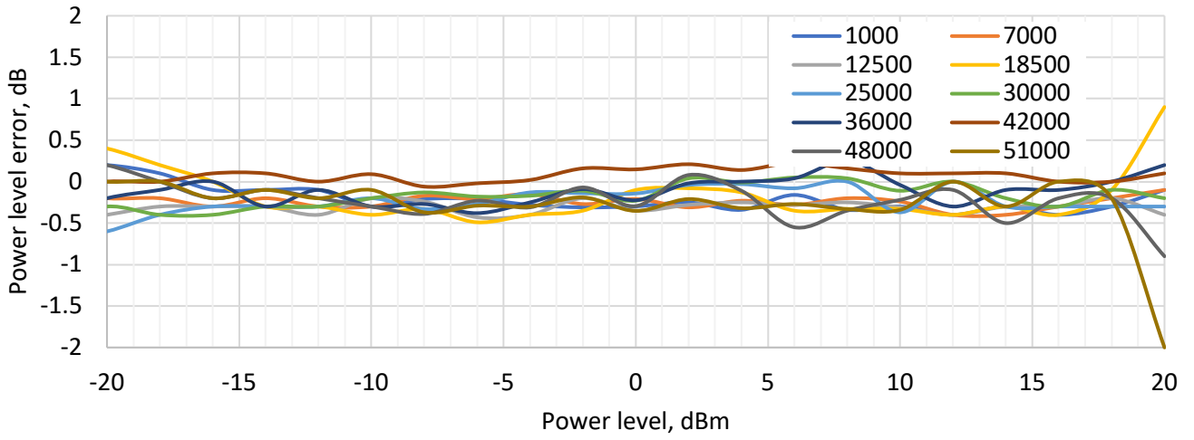
Figure 12: Absolute power level error at different frequencies
