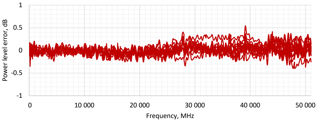
Figure 11: Power level error between -15 and +15 dBm over frequency
