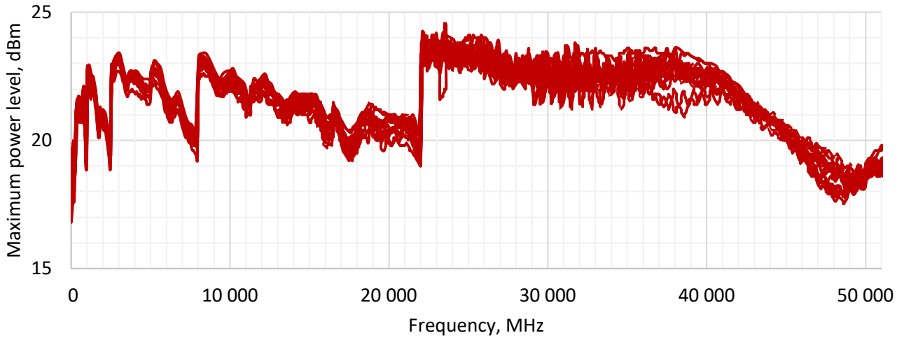
Figure 9: Maximum power level statistics over 20 devices
