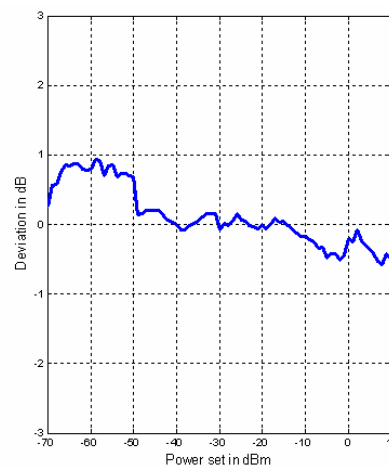
Level Linearity at 2.4 GHz
